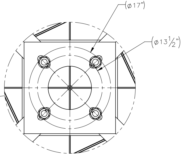
DETAIL B
