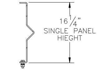
SECTION A-A PANEL PROFILE
