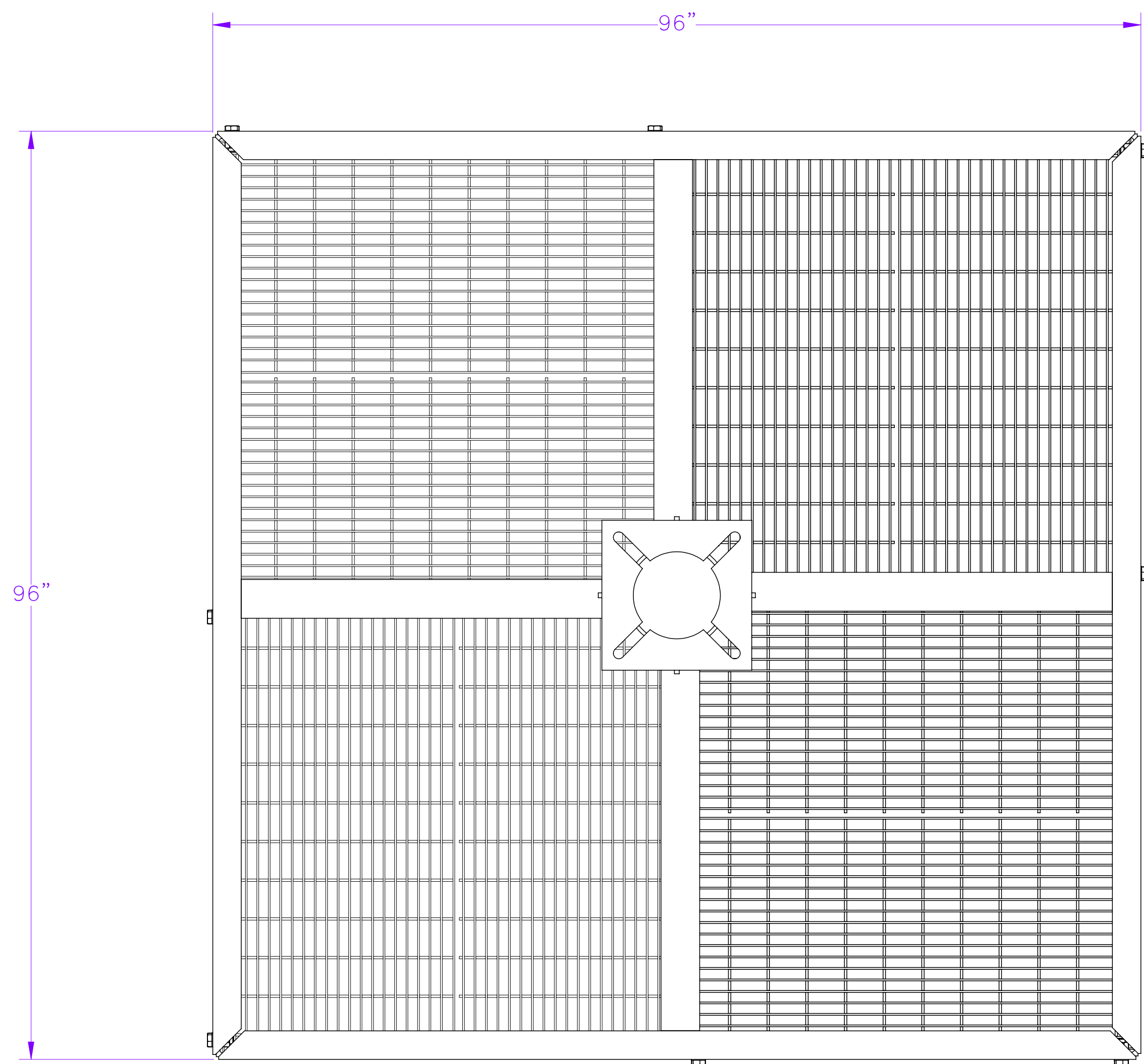
TOP VIEW (SHOWN WITH TOP GRATING REMOVED FOR CLARITY)
