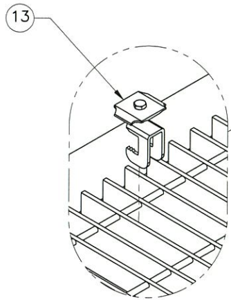
GRATING CLIP DETAIL 4X PER PANEL
