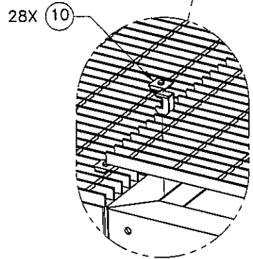
TYP GRATING CLIP DETAIL 4X PER PANEL
