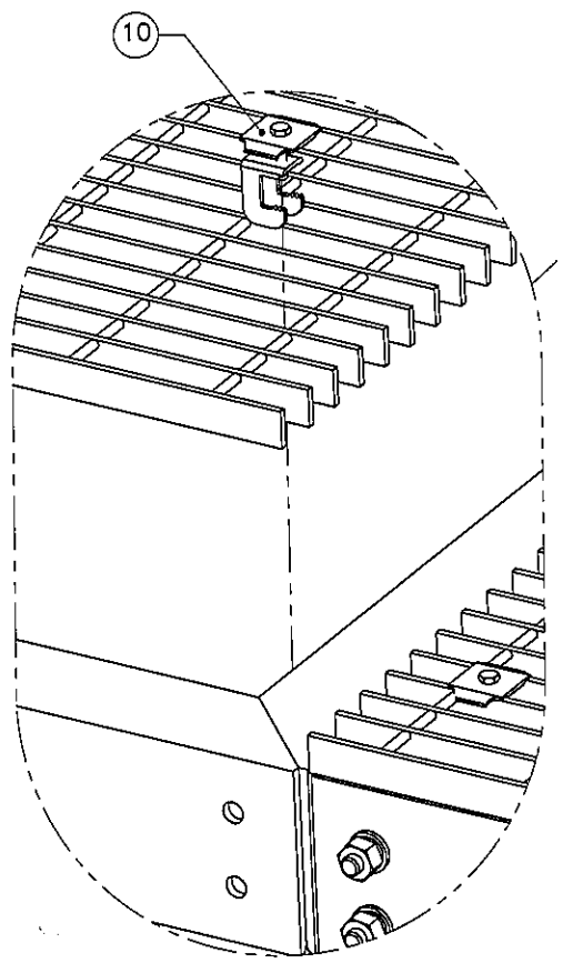
TYP GRATING CLIP DETAIL 4X PER PANEL
