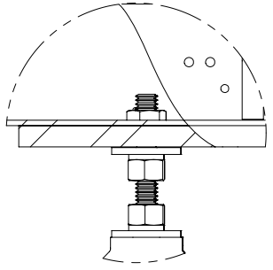
DETAIL A 9 PLCS
